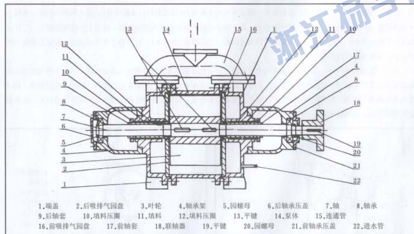
图4 SK-6/12/20/30/42/60/85/120水环泵
